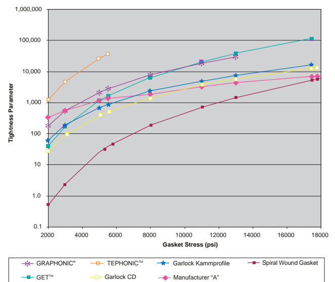
Gasket Stress vs. Tightness Parameter
