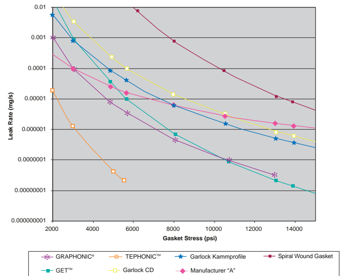
Gasket Stress vs. Leak Rate
